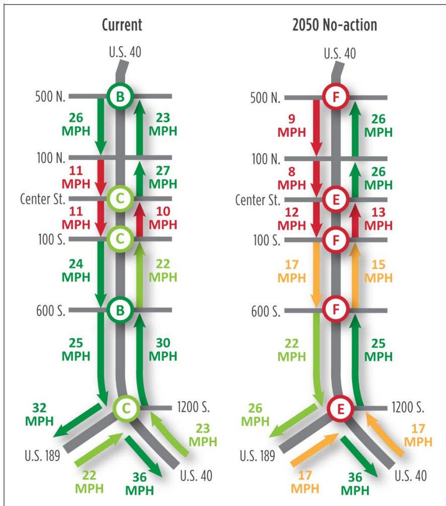
Figure 6. Intersection and Arterial Level of Service on U.S. 40 during the Weekday PM Peak Hour (Current and 2050 No-action)
