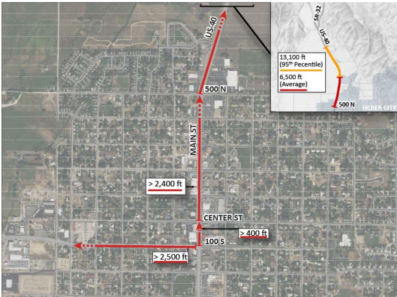
Figure 9. Vehicle Queue Lengths at Key Intersections in the Needs Assessment Evaluation Area during the 2050 No-action PM Peak Hour
